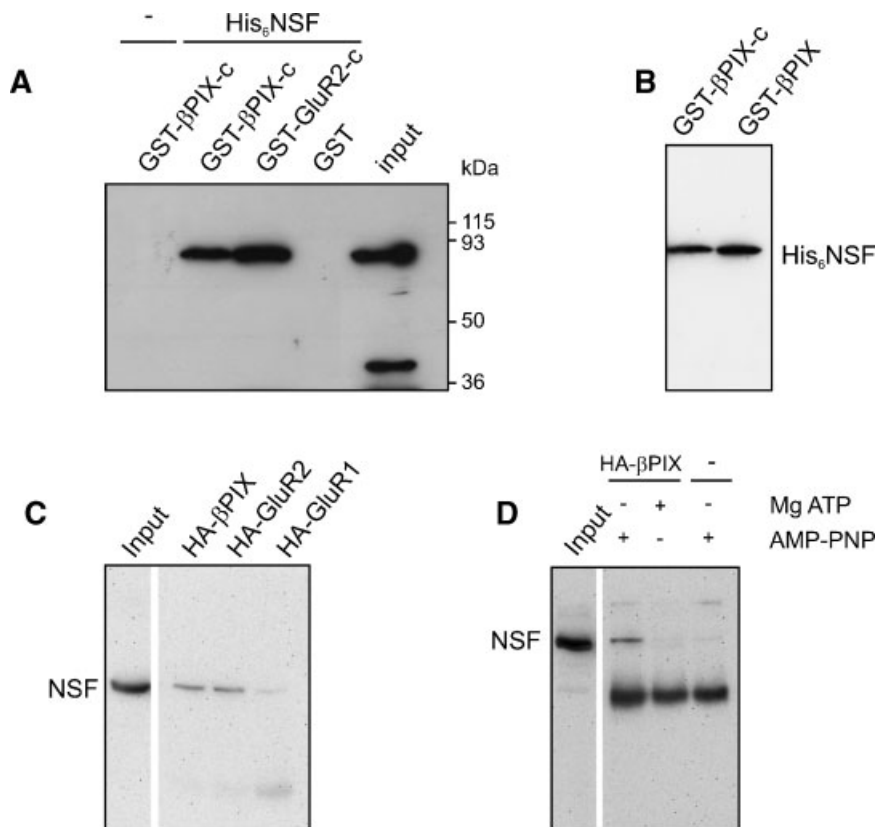
Fig. 1. NSF interacts with the PAK binding exchange factor \beta PIX in vitro and in vivo. GST fusion proteins of isolated yeast two-hybrid \beta PIX clone (GST- \beta PIX-c) and the C-terminus of GluR2 (GST-GluR2-c) were immobilized on glutathione-sepharose for 'pull-down' assays. A: With anti-his antibody a band corresponding to the size of NSF is detected from the lysates of his 6 NSF expressing bacteria, which is precipitated by GST-GluR2-c and GST- \beta PIX-c. No such band is seen with GST alone and no protein is detected with GST- \beta PIX-c pull-down of bacterial lysates not expressing his 6 NSF (-). B: Purified recombinant his 6 NSF is also susceptible to retention by immobilized GST-
