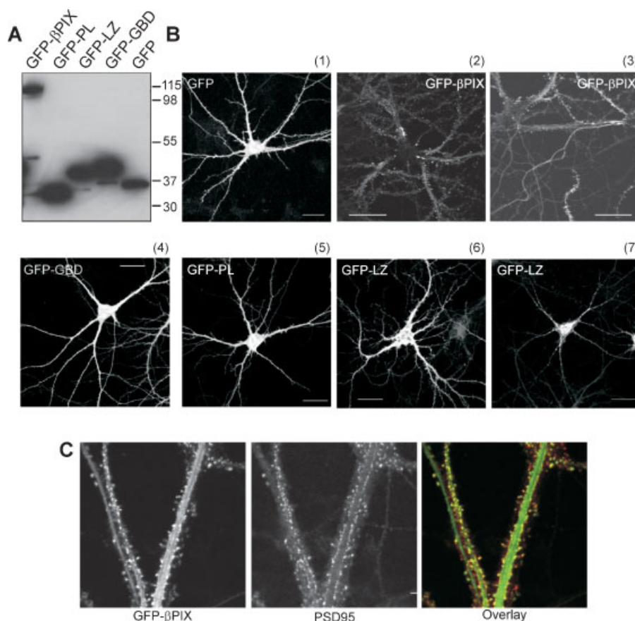
Fig. 3. GFP- \beta PIX is concentrated in spines and axons in cultured hippocampal neurons. A: Full-length \beta PIX and the three C-terminal interaction domains of \beta PIX were expressed as GFP fusion proteins in primary hippocampal cultures through Sindbis virus infection. Cell lysates from infected neurons were probed for expression of GFP fusion protein expression by Western blotting with anti-GFP antibody 24 h after infection. B: GFP signals from 2 to 3 weeks in vitro infected neurons. In comparison to GFP, GFP- \beta PIX is found in a punctate distribution particularly
