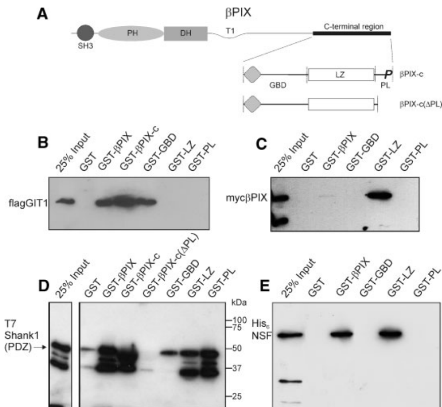
Fig. 2. NSF binds to \beta PIX via its LZ domain. A: Schematic diagram of \beta PIX indicating the arrangements of the src-homology 3 (SH3), pleckstrin-homology (PH), Dbl-homology (DH) and regulatory (T1) domains. The C-terminal region of \beta PIX may be divided into three regions; the GIT-binding domain (GBD), coiled-coil leucine zipper domain (LZ) and PDZ ligand domain (PL). B: Immobilized GST fusion proteins containing the GBD are able to retain recombinant Flag-GIT1 from HEK293 cell lysates, detected by anti-flag Western blot. C: \beta PIX is reported to dimerise through its LZ domain. Consistent with this an immobilized GST fusion protein comprising the LZ region retains recombinant
