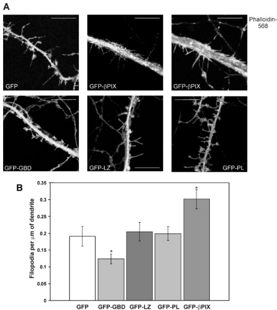
Fig. 4. The formation of dendritic filopodia is promoted by \beta PIX expression, but is insensitive to expression of NSF interaction domain. A: Cultured hippocampal neurons 11–14 days in vitro infected for 18 h with GFP- \beta PIX or GFP- \beta PIX C-terminal interaction domains. Fluorescent images are of short sections of dendrites from infected neurons. Protrusions are seen projecting off the dendrite with all GFP fusion constructs, however GFP- \beta PIX-induced protrusions may be better seen using the actin stain
